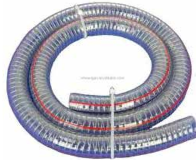
1inch, 25mm inner diameter, 250Psi, high temperature braided flexible iron, high abrasion resistant cover
